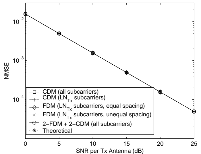
Fig. 1. The NMSEs of several optimal training structures for an MIMO OFDM system with N_{Tx} = 4 , K = 64 in an 8-tap multipath Rayleigh fading channel with an exponential power delay profile
