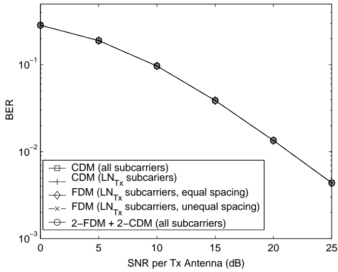
Fig. 2. The BERs of several optimal training structures for an MIMO OFDM system with N_{Tx} = 4 , K = 64 in an 8-tap multipath Rayleigh fading channel with an exponential power delay profile
