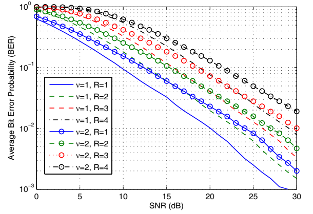
Fig. 2. Average detection error probability in two-tap and three-tap ISI channels with ZF linear equalization.
