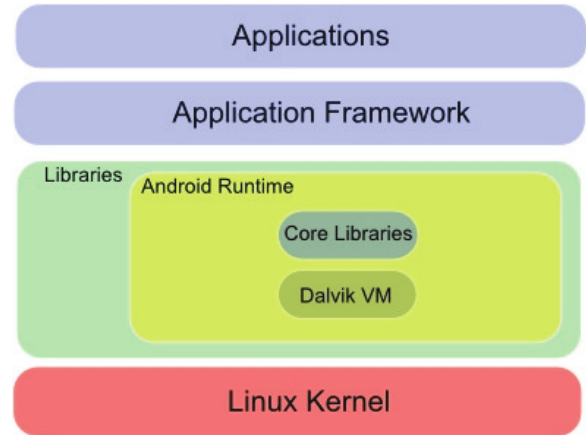
Figure 1. Android Architecture
