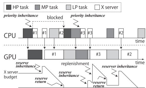
Figure 10. Example of RIX procedure.
