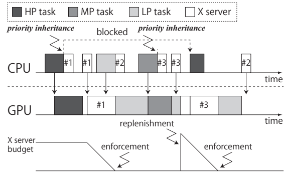
Figure 9. Example of untimely enforcement in the GPU-accelerated X Window System.
