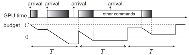
Figure 5. Example of GPU reservation [27].
