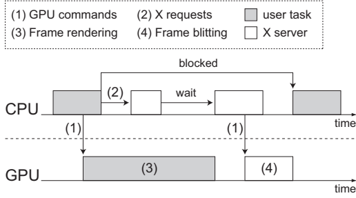
Figure 6. Interaction between a user task and the X server in the DRI-based X Window System.
