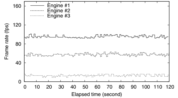
Figure 2. Frame-rates of three graphics tasks with priorities lower than the X server in the presence of an X-client task.
