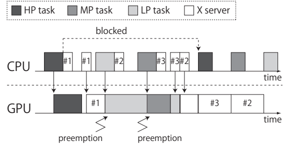
Figure 7. Example of priority inversion in the GPU-accelerated X Window System.
