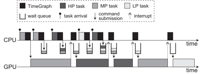
Figure 4. Example of GPU scheduling [27].
