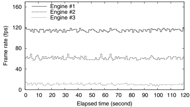
Figure 14. Frame-rates of three graphics tasks in the presence of an X-client task under PIX.
