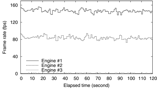
Figure 1. Frame-rates of three graphics tasks with priorities lower than the X server.
