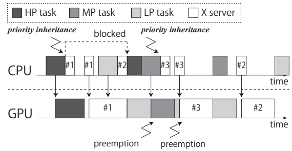
Figure 8. Example of PIX procedure.
