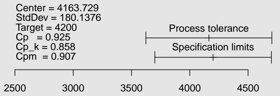
Capability plot
