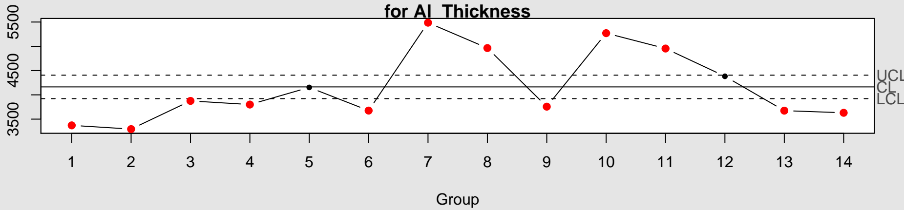
R Chart for Al Thickness
