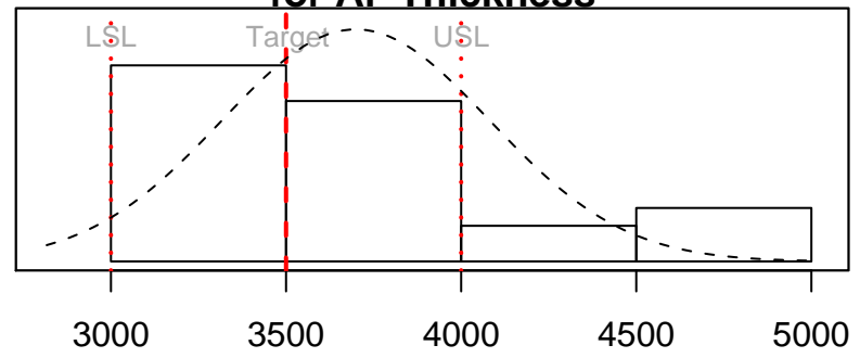
Process Capability Analysis for Al Thickness
