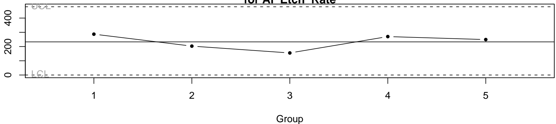
R Chart for AI Etch Rate
