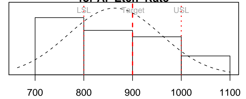
Process Capability Analysis for AI Etch Rate
