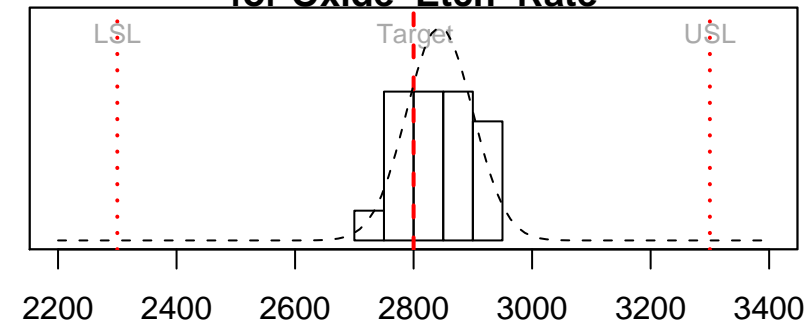
Process Capability Analysis for Oxide Etch Rate
