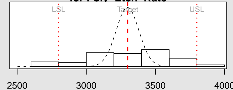
Process Capability Analysis for Poly Etch Rate
