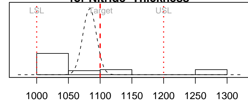
Process Capability Analysis for Nitride Thickness
