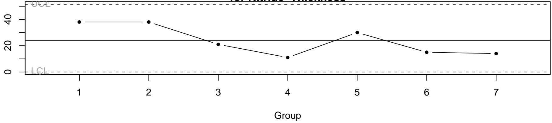
R Chart for Nitride Thickness
