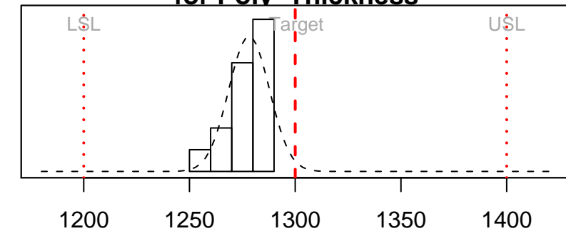
Process Capability Analysis for Poly Thickness
