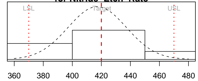
Process Capability Analysis for Nitride Etch Rate
