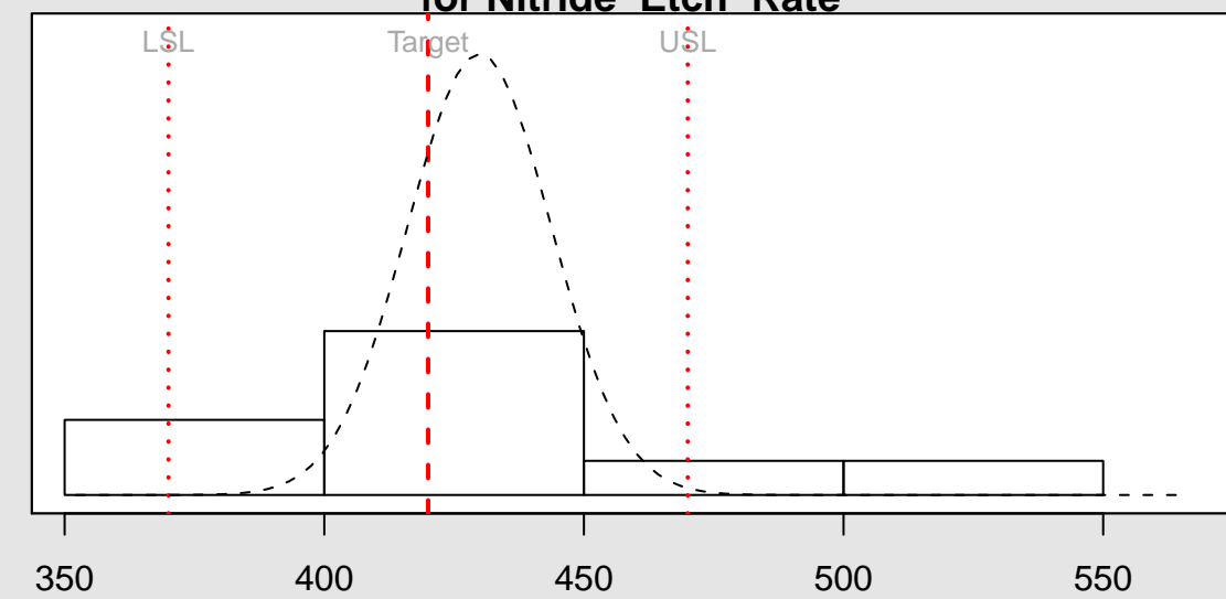
Process Capability Analysis for Nitride Etch Rate
