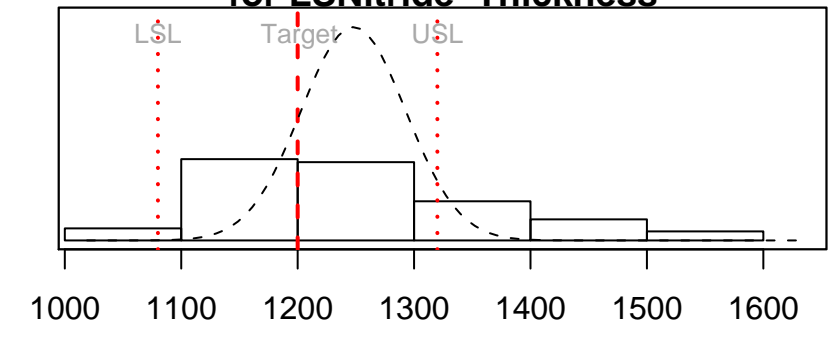
Process Capability Analysis for LSNitride Thickness
