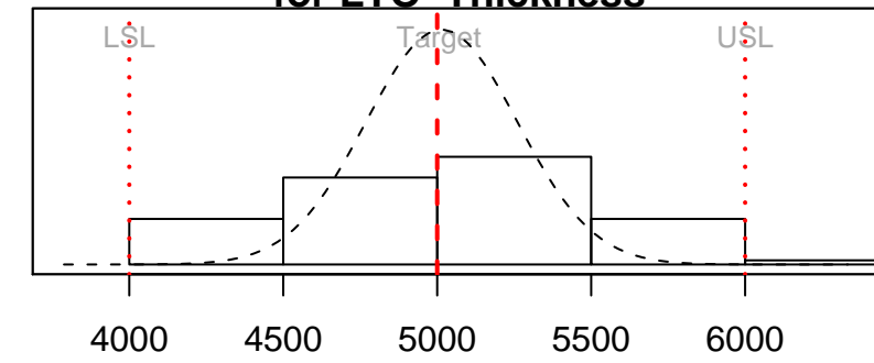
Process Capability Analysis for LTO Thickness
