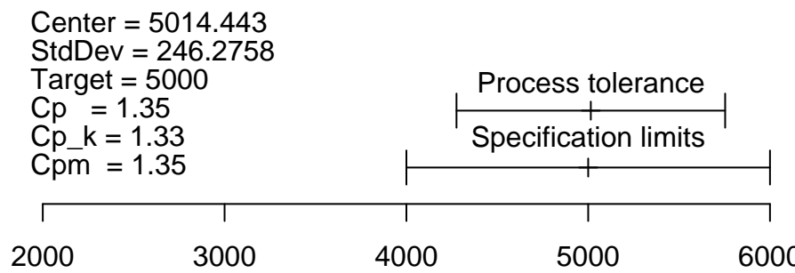
Capability plot
