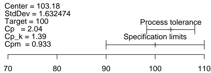
Capability plot
