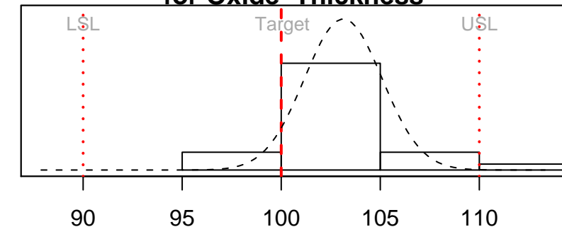
Process Capability Analysis for Oxide Thickness
