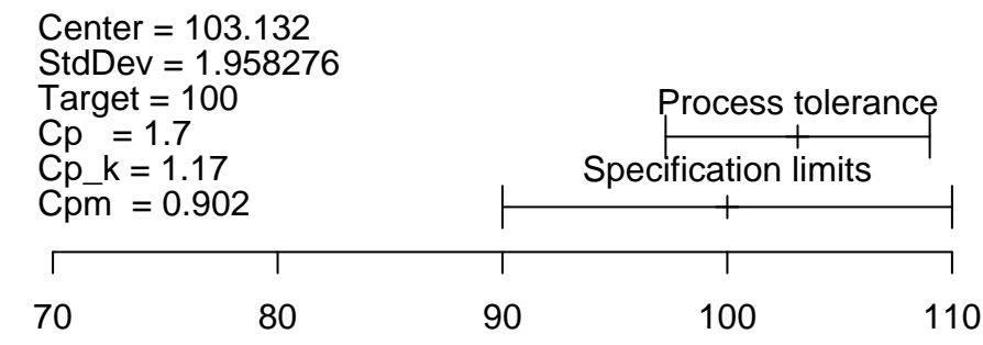
Capability plot
