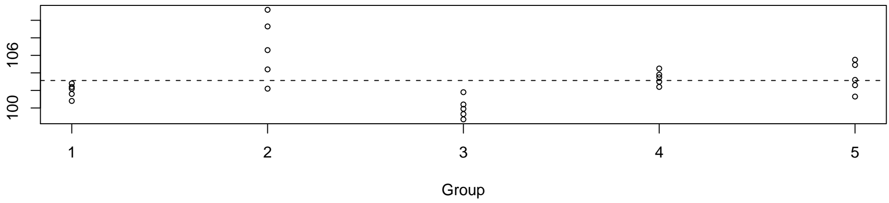
Run chart
