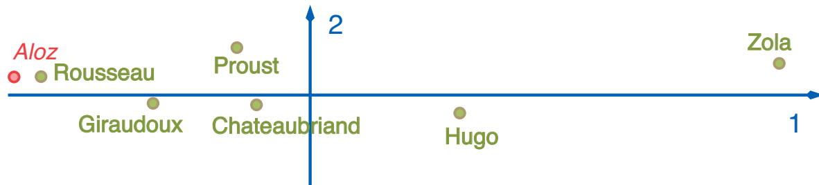
Figure 1: PCA analysis of the Punctuation. Centered Data. Alos is a supplementary element. Even though Alos punctuates the same way as Zola, Alos is further away from Zola than any other author. The first dimension explains 98% of the variance. It reflects mainly the number of punctuation marks produced by the author.
