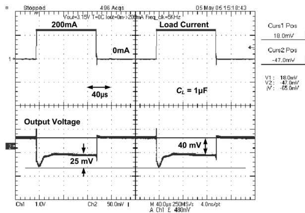
Fig. 12. Measured load transient response of the proposed LDO for a load step pulsating between 0 and 200 mA with rise and fall time of 100 ns and V_{out} = 3.15\text{ V} .
