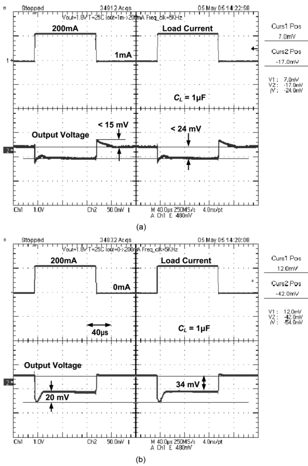
Fig. 11. Measured load transient response of the proposed LDO for a load step pulsating (a) between 1 mA and 200 mA and (b) between 0 and 200 mA with rise and fall time of 100 ns and V_{out} = 1.8\text{ V} .
