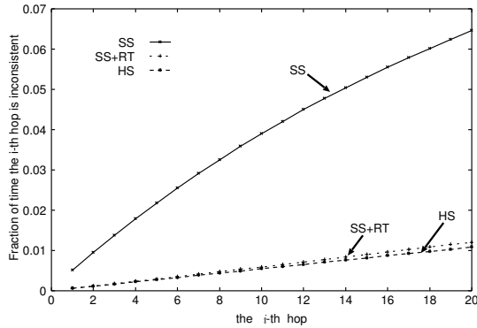
Figure 13: Fraction of time that the i -th hop is inconsistent, where 1 \leq i \leq N and N = 20
