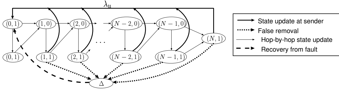
Figure 12: Markov model for hard-state signaling approach
