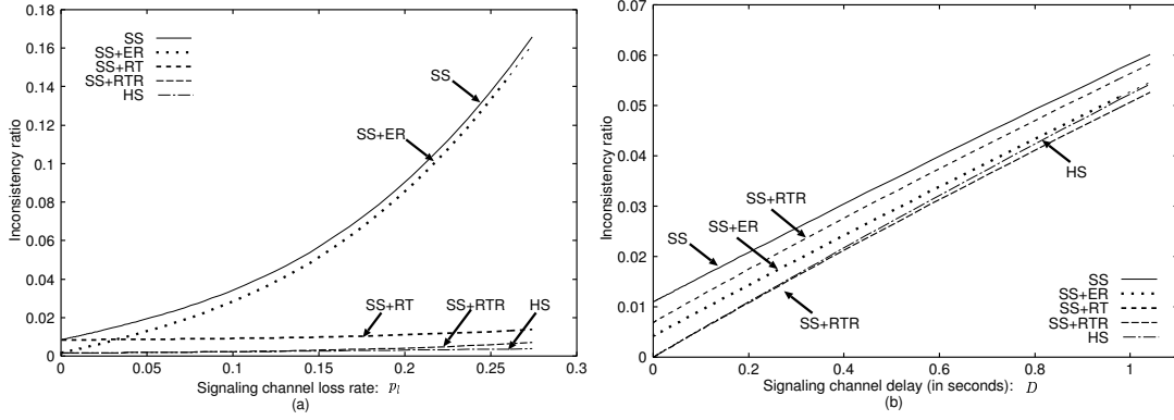
Figure 5: Comparison against link loss rate p_l and link delay D
