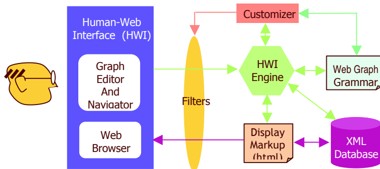
Figure 3: The HWI framework
