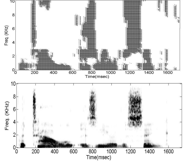
Fig 1: Top panel: Plot of estimated speech presence probability based on the ratio S_r(\lambda, k) . Bottom panel: spectrogram of the clean signal.
