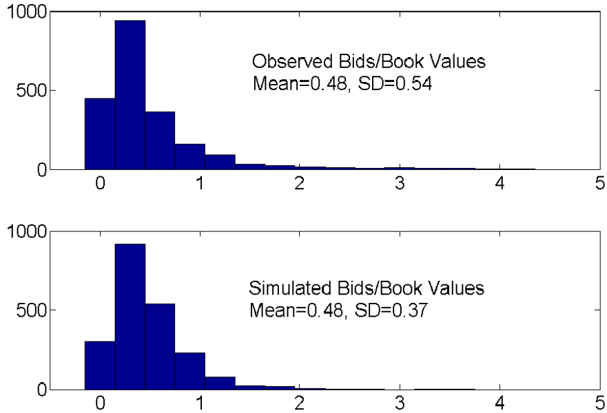
Figure 4: Observed Bids Vs. Simulated Bids
