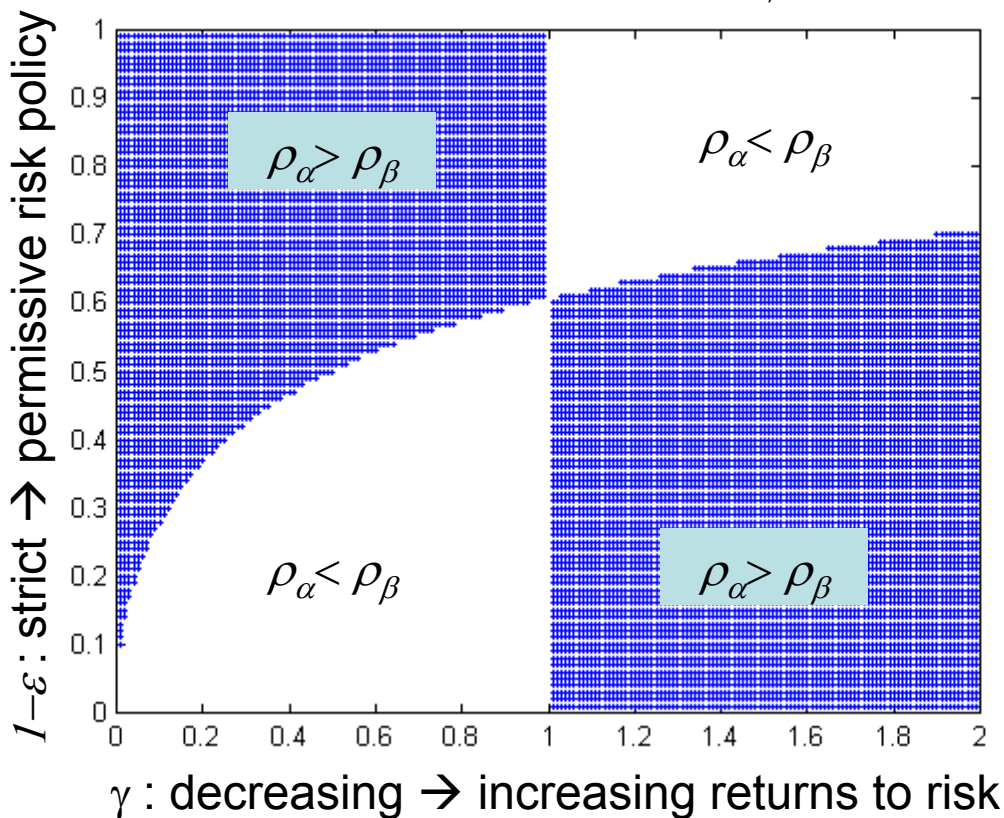
Figure 1: Shaded region depicts environment-policy pairs (\gamma, I-\varepsilon) for which the hypothesis of satisficing ( \alpha ) provides a greater rationale for paternalism (\rho_\alpha > \rho_\beta)^*
