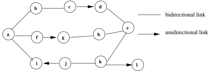
Figure 2. Ad hoc network with unidirectional and bidirectional links.
