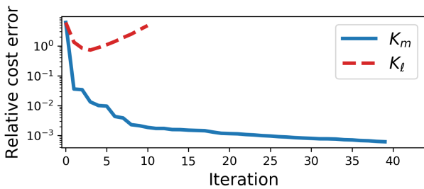
Fig. 1. Relative LQRm cost error \frac{C(K) - C(K^*)}{C(K^*)} vs. iteration during policy gradient descent on the 4-state, 1-input suspension example system.
