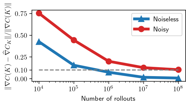
Fig. 3. Relative gradient estimation error vs. number of rollouts for (13).
