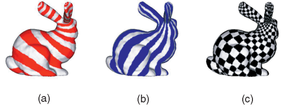
Fig. 4. The global conformal parameterization of the bunny model.
