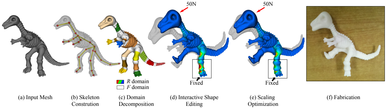
Figure 1: The workflow of our system. (a) The input of our system is a tetrahedral mesh. (b) A skeleton is constructed from the input mesh. (c) The mesh is decomposed to domains according to the skeleton, and the decomposed domain is associated with the bones. (d) Users can edit the mesh and see the influence on stress distribution interactively. (e) Our system also can optimize the shape to reduce stresses. (f) After the stresses are reduced to a safe level, the edited mesh is used to print real objects.
