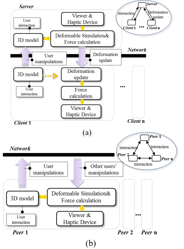
Fig. 2. Proposed collaborative system over (a) the Client-Server (C-S) and (b) the Peer-to-Peer (P2P) architectures.
