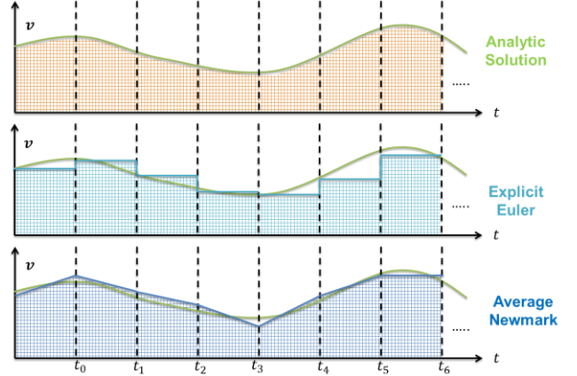
Fig. 5. Numerical integration over time assumes either velocity or acceleration to be constant within one time-step.
