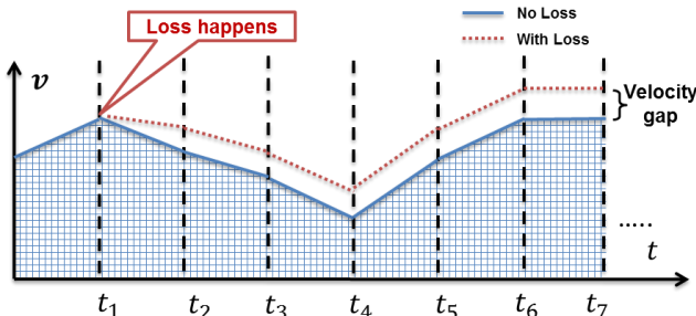
Fig. 4. Displacement and velocity errors along time. When data is lost at t_1 , velocity changes along red dash line.
