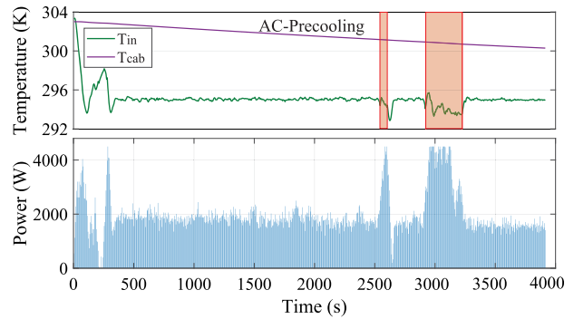
Fig. 13 The A performance with MPC-based energy management
