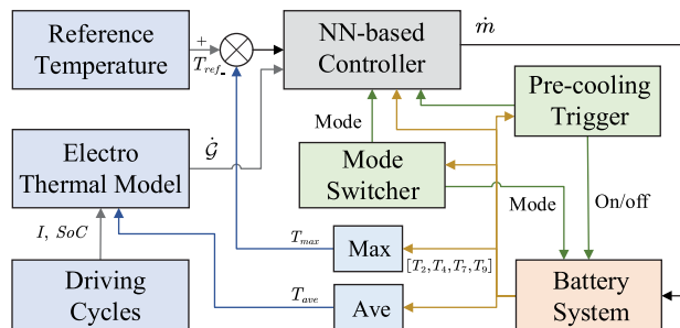
Fig. 6 The control framework of the air-based J-type BTMS
