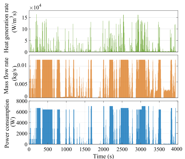
Fig. 8 The BTMS properties without energy management
