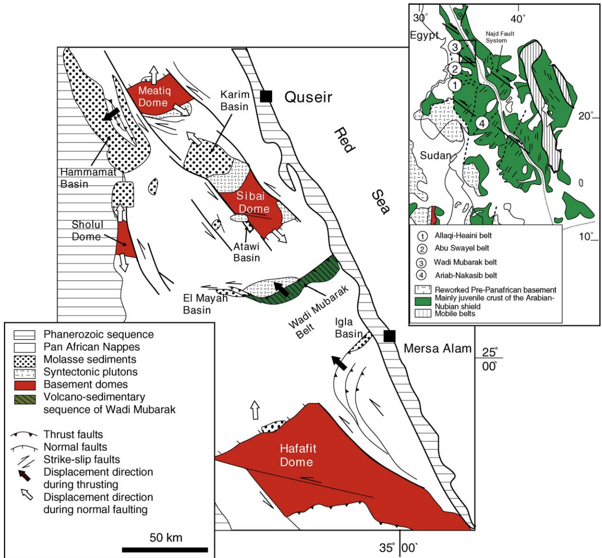
Fig. 1. Tectonic map of the Central Eastern Desert showing the core complexes, the northwest–southeast striking Najd fault system and the location of the Wadi Mubarak belt (modified after Fritz et al., 1996). The inset shows the Najd Fault System and other deformation belts in the Arabian–Nubian Shield.
