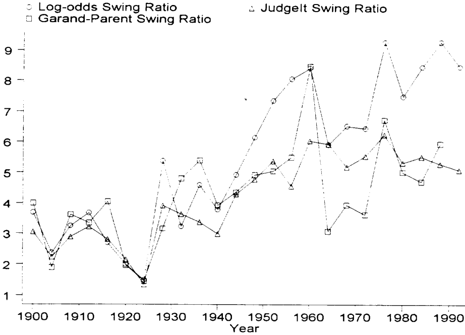
Fig. 1. Swing ratio in the electoral college, 1900–1992. The methods of calculating each measure of the swing ratio are described in the text
